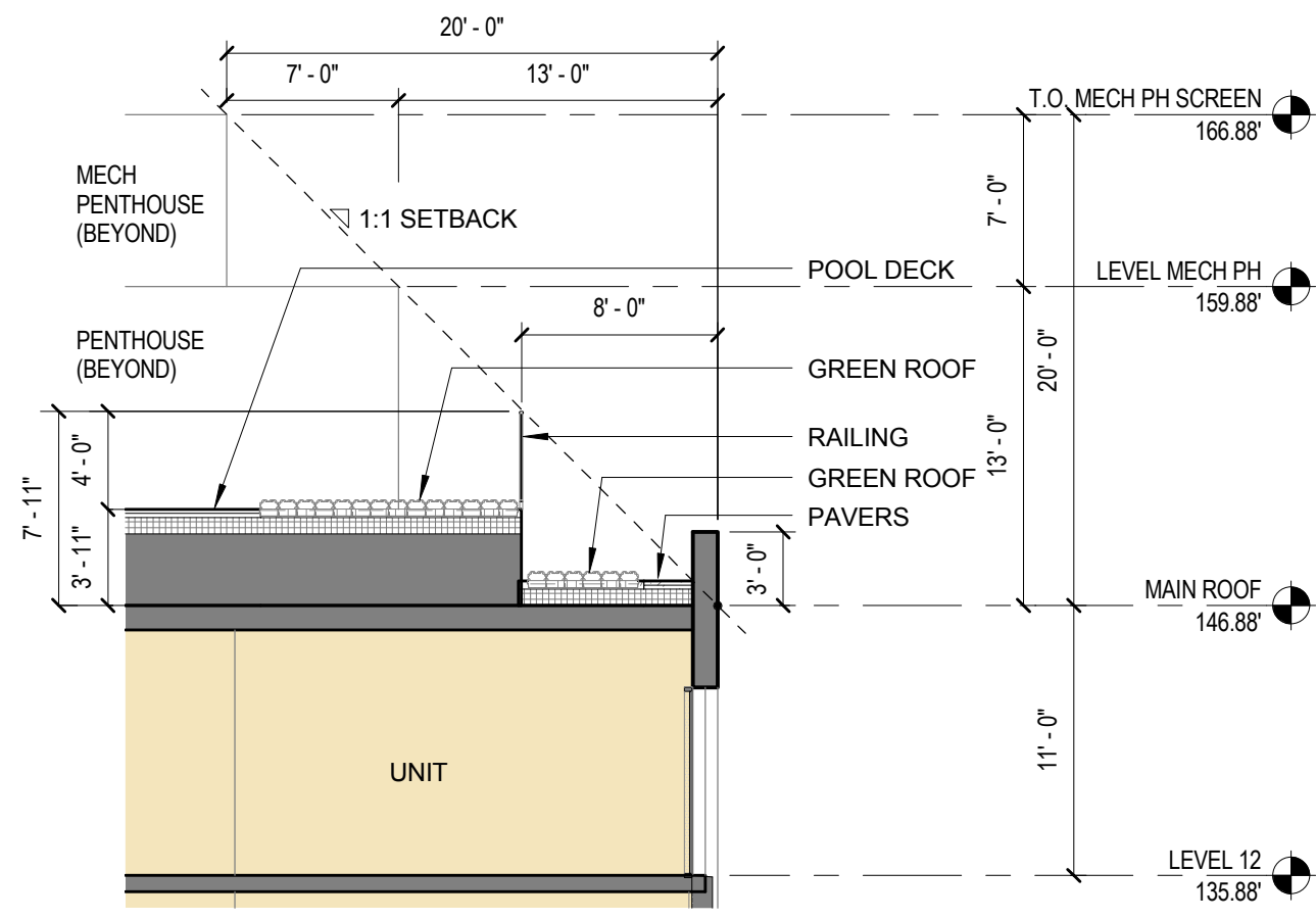
2 ENLARGED SECTION 2 1/8" = 1'-0"
